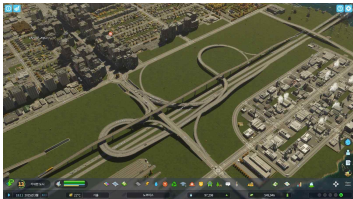
Cities: Skylines
